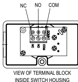
Figure 2: Wiring Diagram
