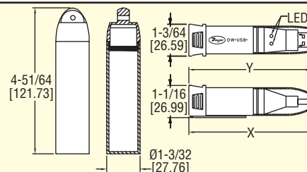
Model DW-USB-CASE
