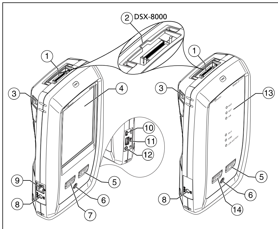
Figure 1. Connectors, Keys, and LEDs (Versiv 2 shown)
