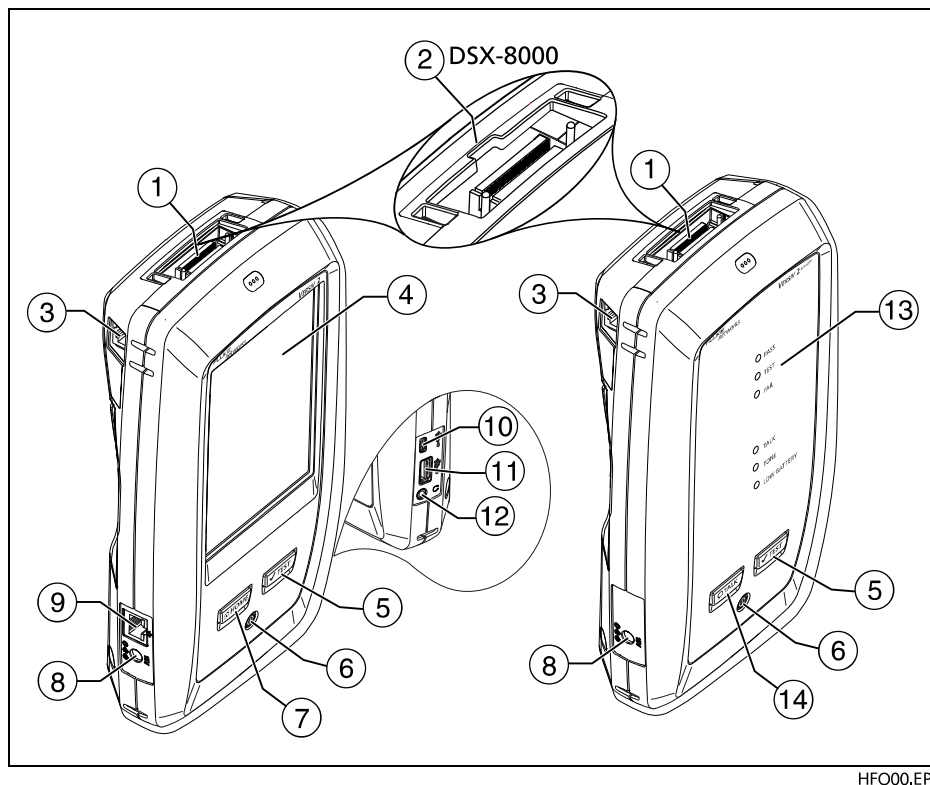
Figure 1. Connectors, Keys, and LEDs (Versiv 2 shown)
