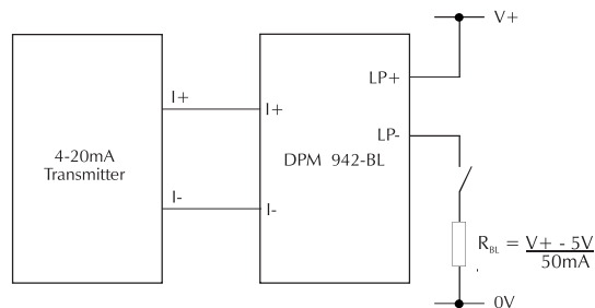
Powering the LED backlighting. The supply voltage for the LED backlighting should be electrically isolated from the 4-20mA current loop.
