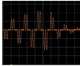
Forming machine load current 50A/div, 10ms/div
