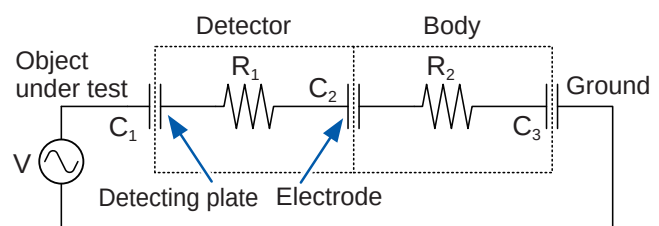
Equivalent circuit diagram
