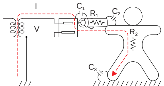
Measuring principle diagram
