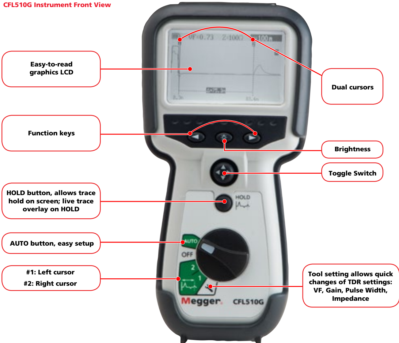
CFL510G Instrument Front View
