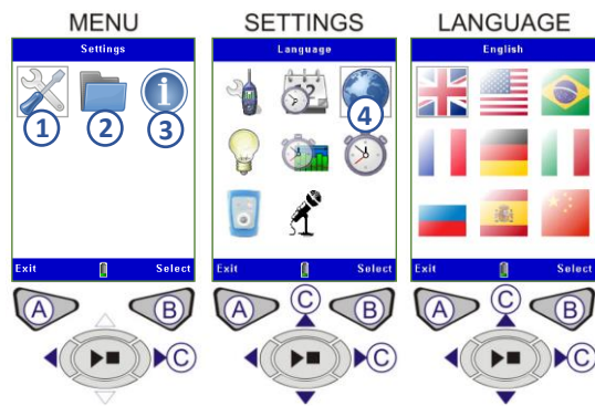
Figure 2 Settings Screen
