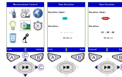
Figure 6 Run Duration
