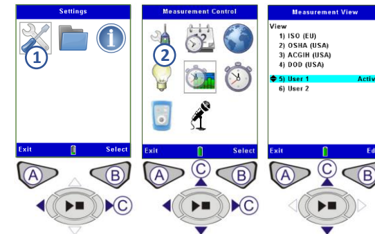
Figure 5 Settings Options
