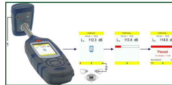
Figure 4 Calibration Screens
