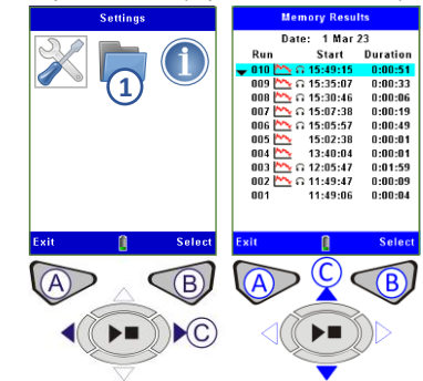
Figure 9 Memory Results
