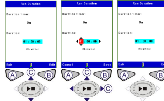
Figure 6 Run Duration
