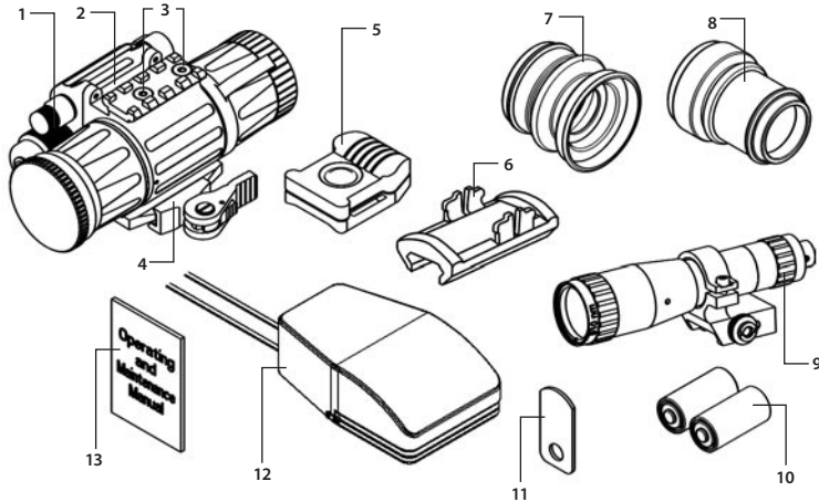
FIGURE 2-3. STANDARD COMPONENTS
