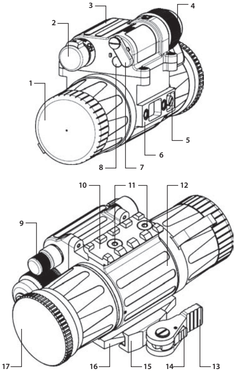
FIGURE 2-2. CO-MINI NIGHT VISION CLIP-ON DEVICE
