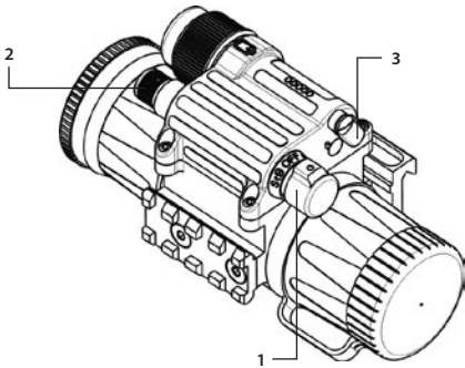
FIGURE 3-14. CO-MINI CONTROLS
