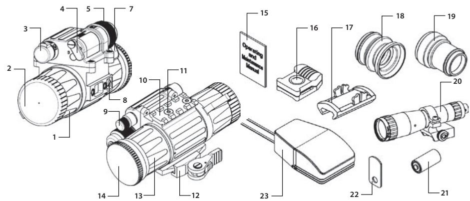
FIGURE B-1. CO-MINI SPARE PARTS
