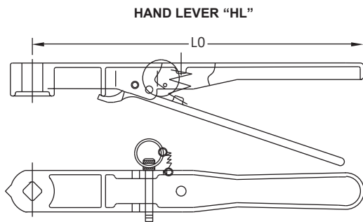
HAND LEVER DIMENSIONS [in (mm)]
