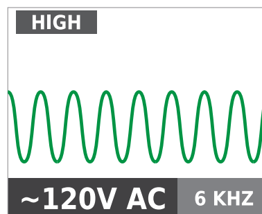
Figure 3.1b Transmitter screen showing signal in HIGH mode with 6kHz frequency for energized circuit
