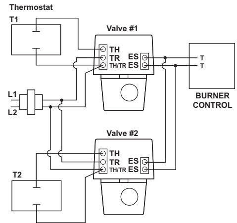
Typical Multiple Valve Wiring
