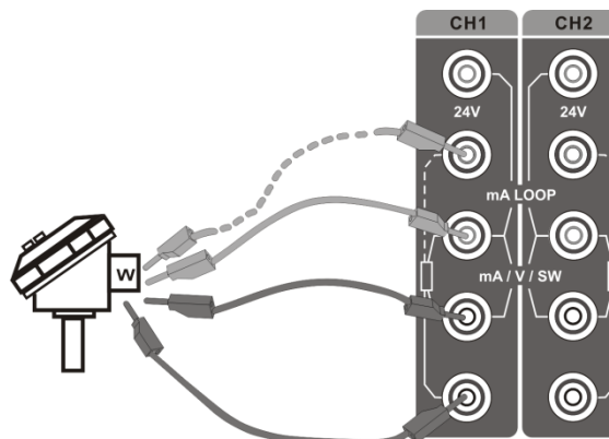
Figure 3 RTD Connection
