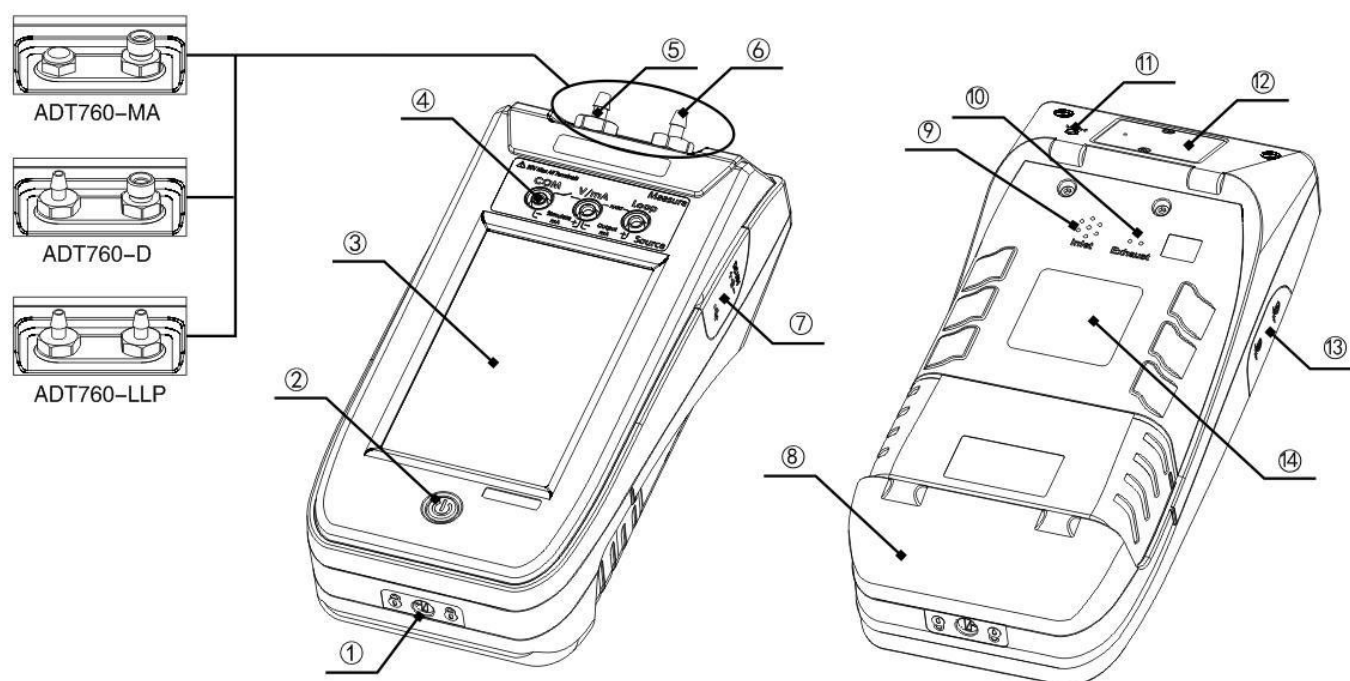
Figure 1 Basic Structure
