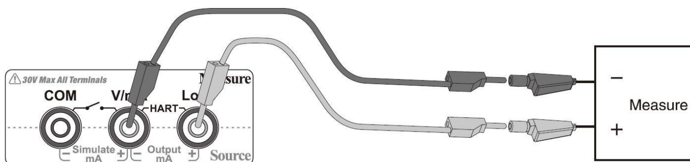
Figure 12 Current Output
