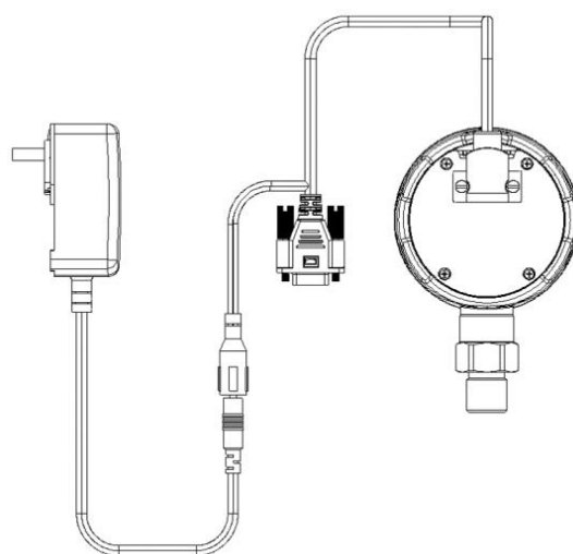
Figure 4 Power supply by adapter
