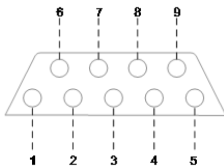
Figure 22 RS232 module DB9 female pins description
