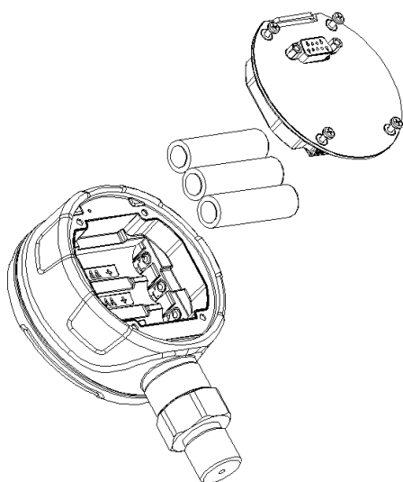
Figure 3 Install batteries
