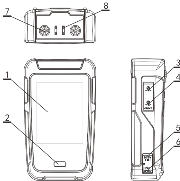
Figure 1 Basic Structure
