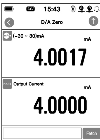
Figure 14 D/A adjustment
