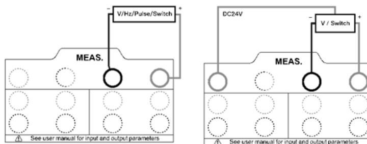
Figure 7 Voltage/ frequency/ pulse/ switch wiring
