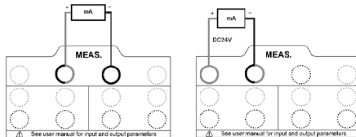
Figure 8 Current measurement
