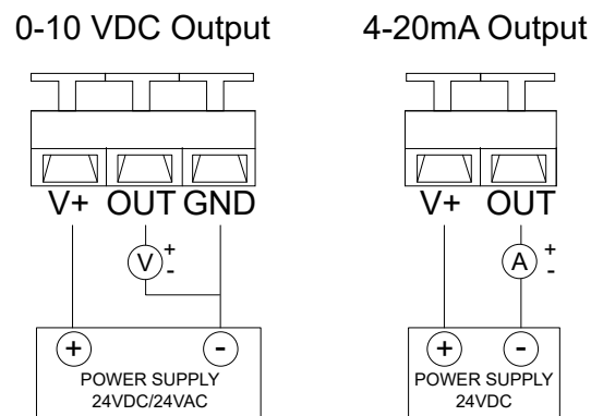
Figure 5 AcuTEMS DM Wiring Terminals for Temperature Transmitter
