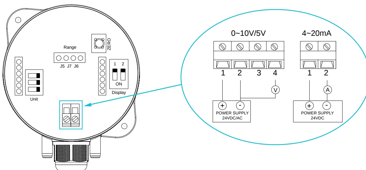
Figure 6 AcuPRE DM Wiring Terminals
