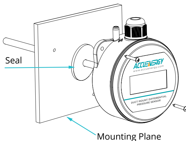
Figure 3 Direct Duct Mount for AcuPRE DM
