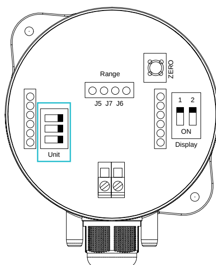
Figure 8 AcuPRE DM Unit Selection DIP Switches
