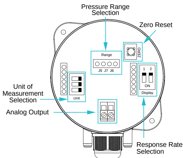
Figure 2 Internal Schematics of AcuPRE DM
