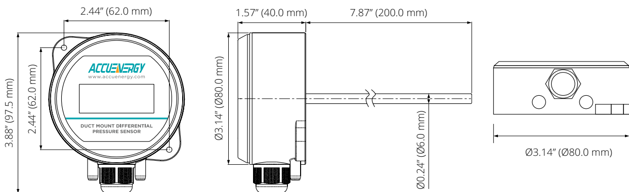
Figure 1 AcuPRE WM Front and Bottom Views
