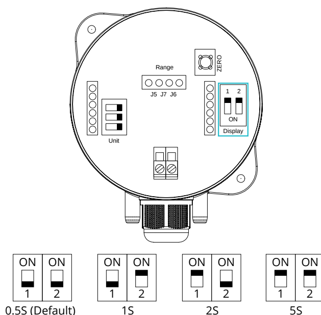
Figure 9 AcuPRE DM Response Time Selection DIP Switches
