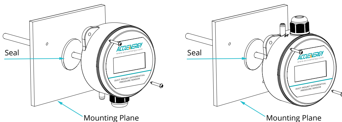
Figure 5 AcuPRE DM Installed with Cordgrip Facing Upward and Downward
