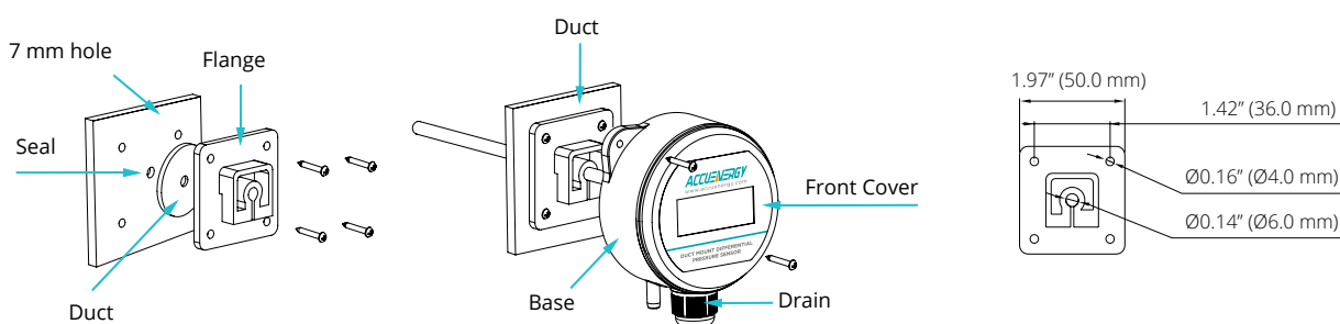
Figure 4 Duct Mount with Flange
