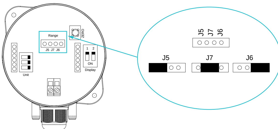
Figure 7 AcuPRE DM Pressure Range Selection Jumpers
