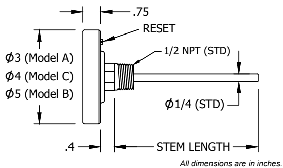
Standard Dimensions
