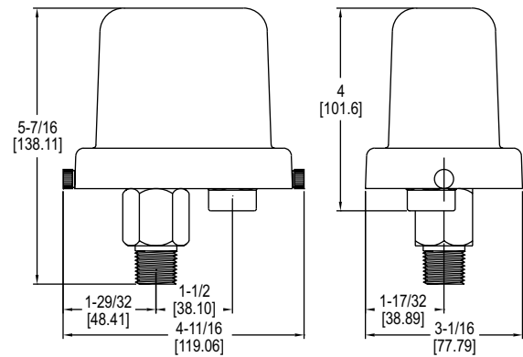
A1F with -PC weatherproof housing
