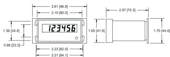
Base Mount
