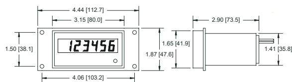
Panel Mount
