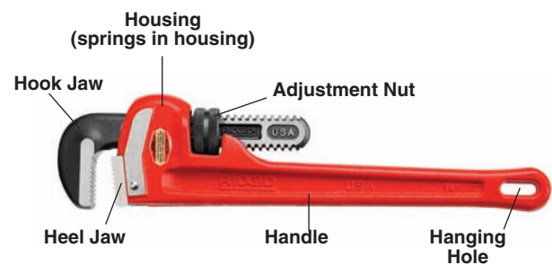
Figure 2 – Wrench Parts
