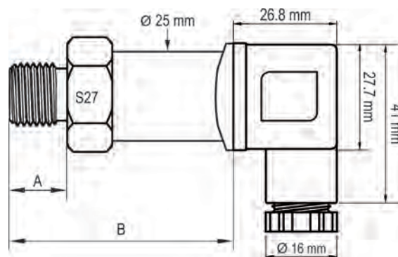
Figure 3 – Transmitter dimensions
