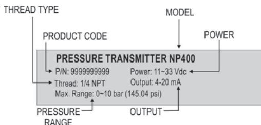
Figure 1 – Transmitter identification
