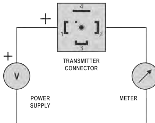
Figure 2 – Electrical connections
