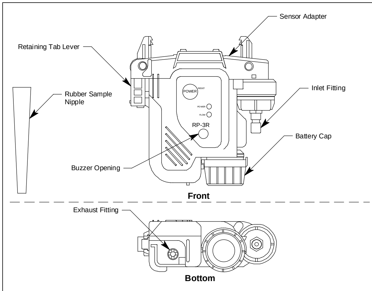
Figure 1: Component Location
