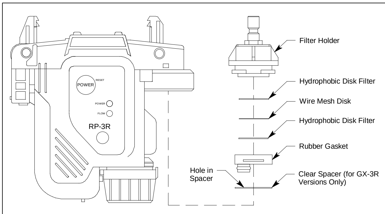
Figure 5: Changing the Hydrophobic & Wire Mesh Filters
