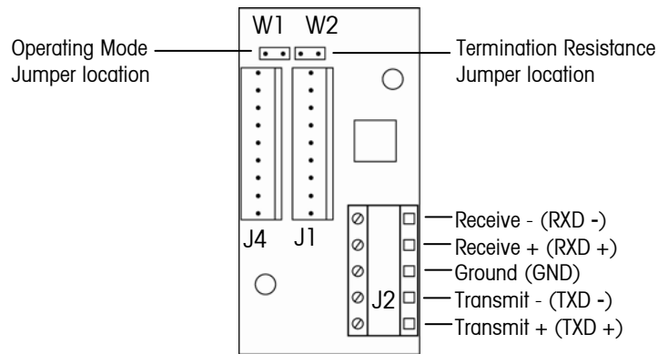
Figure 2.2 RS485 Connections
