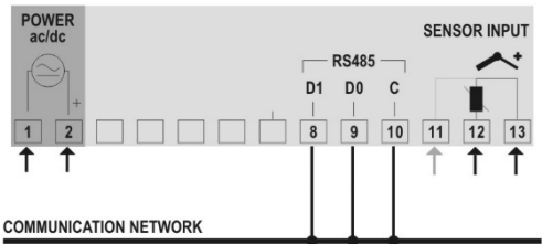
Figure 01 – Communication connections
