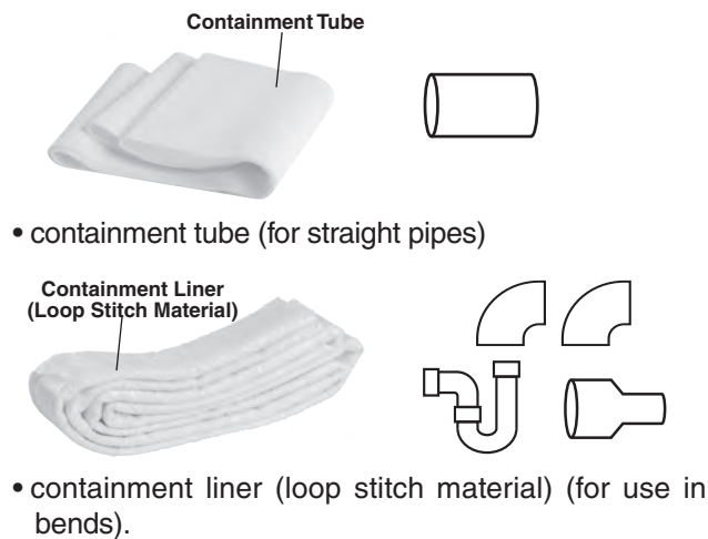
Figure 19 – Containment Examples
