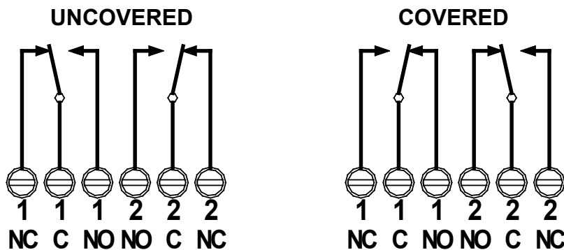
FAIL-SAFE “LOW” RELAY CONTACT POSITION
