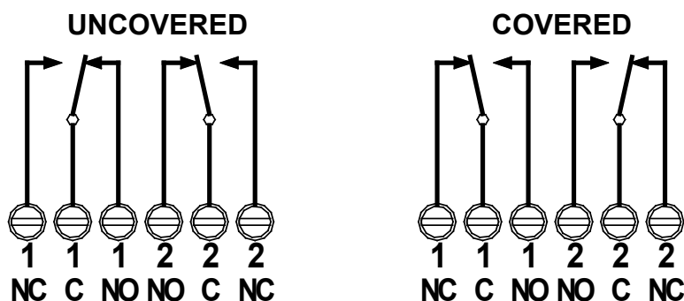
FAIL-SAFE “HIGH” RELAY CONTACT POSITION
