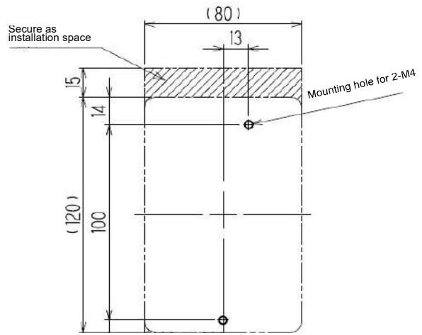
Installation dimension drawing (Installation board used)
