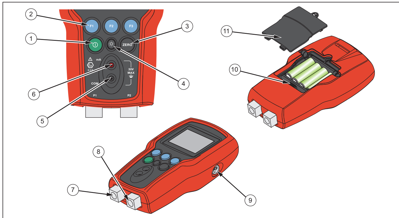
Figure 1. Product Interface
