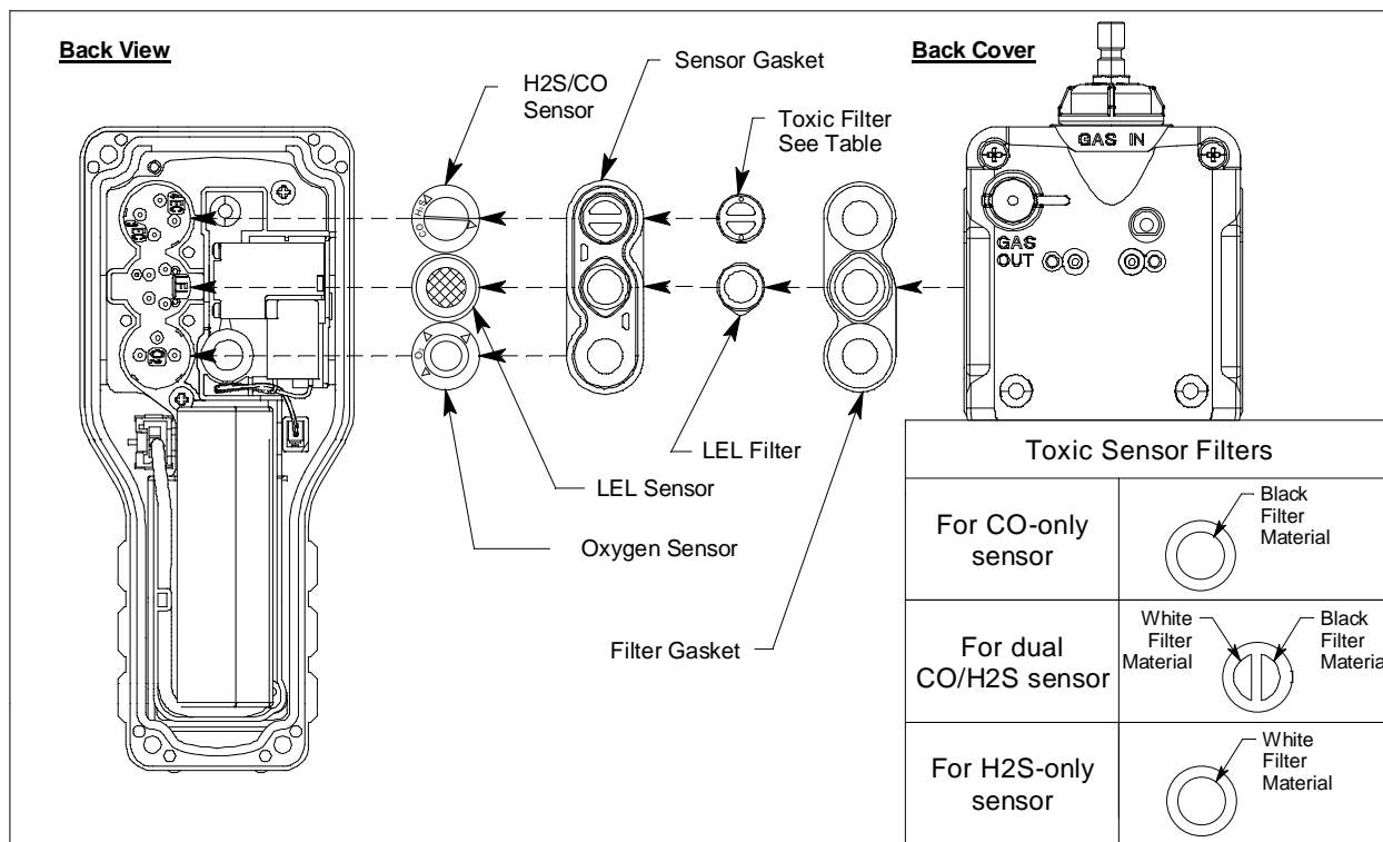
Figure 11: Replacing a Sensor
