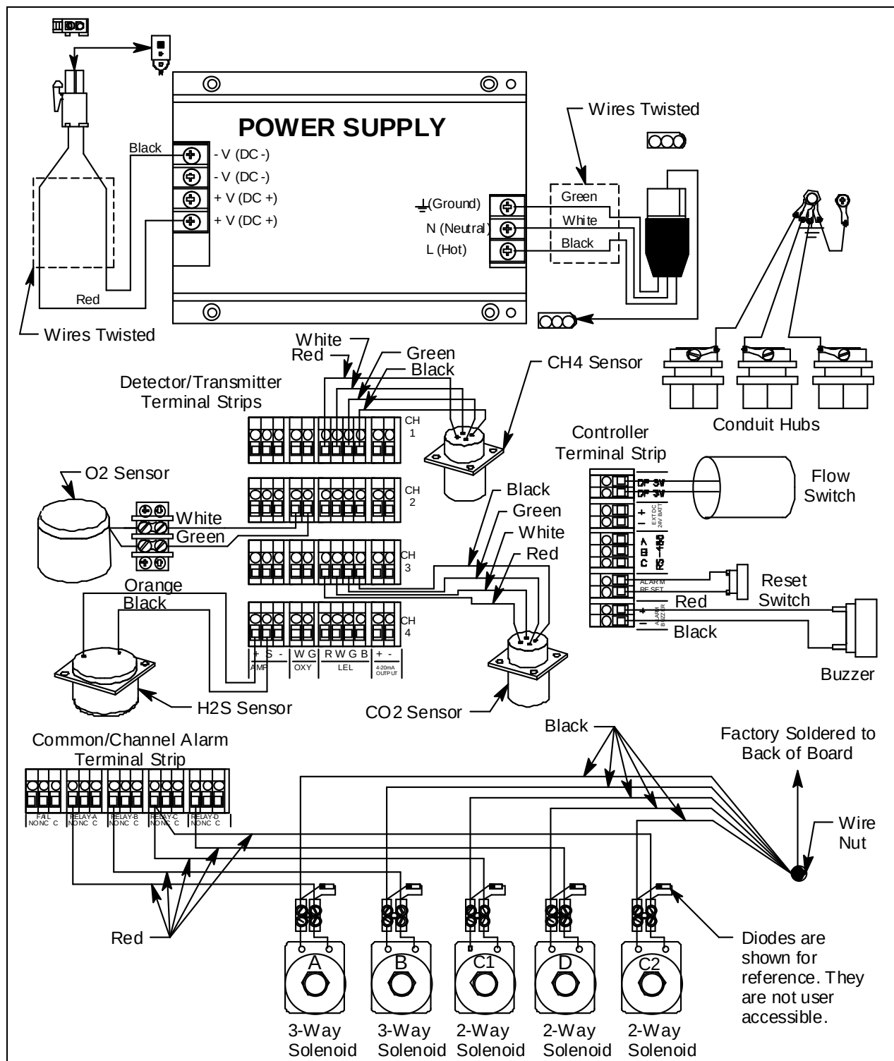
Figure 7: Factory Wiring
