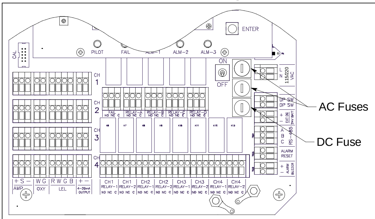
Figure 45: Fuse Location
