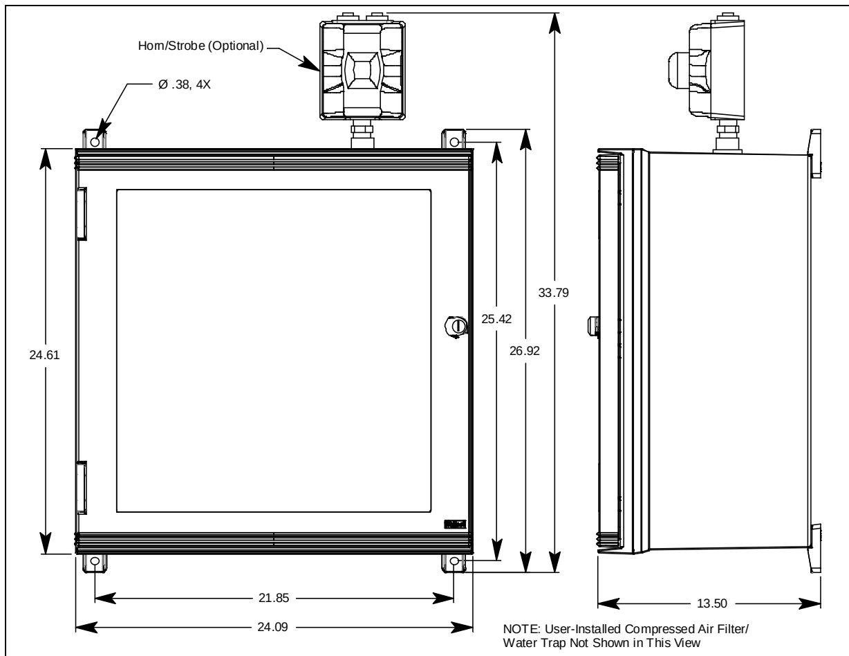
Figure 11: Mounting Dimensions
