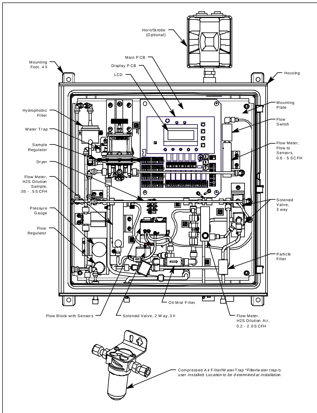
Figure 3: Internal Component Location
