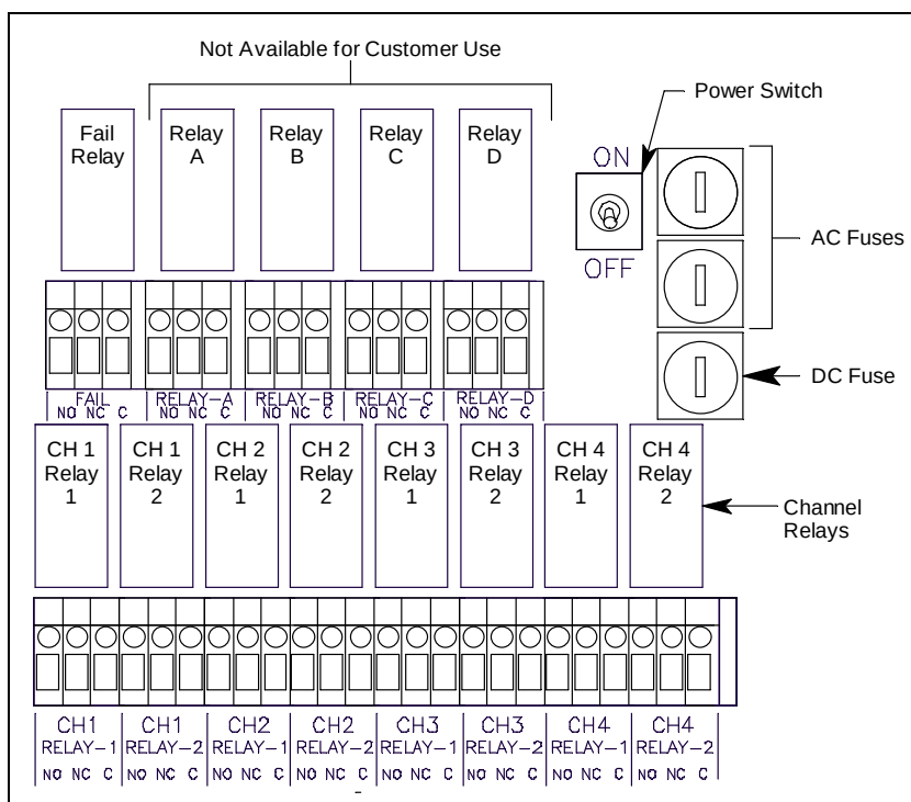
Figure 6: Relay Allocation
