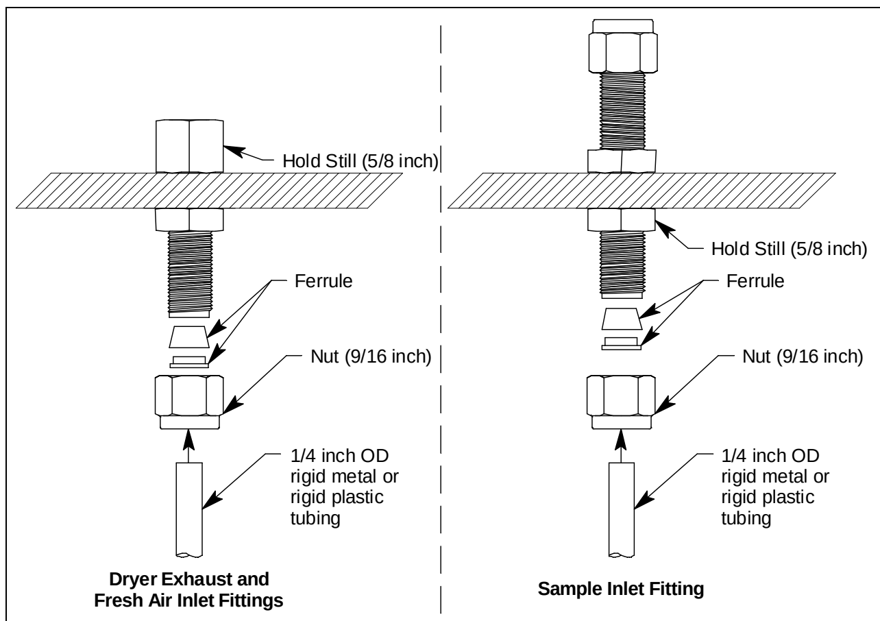
Figure 19: Compressed Fitting Connection
