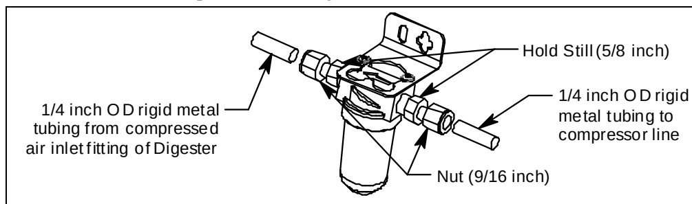
Figure 18: Compressed Air Filter/Water Trap
