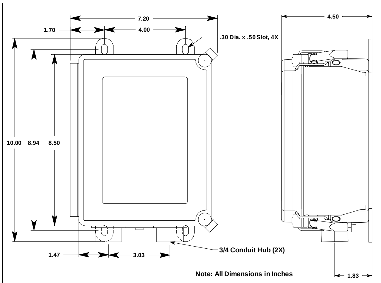
Figure 6: Beacon 110 Dimensions
