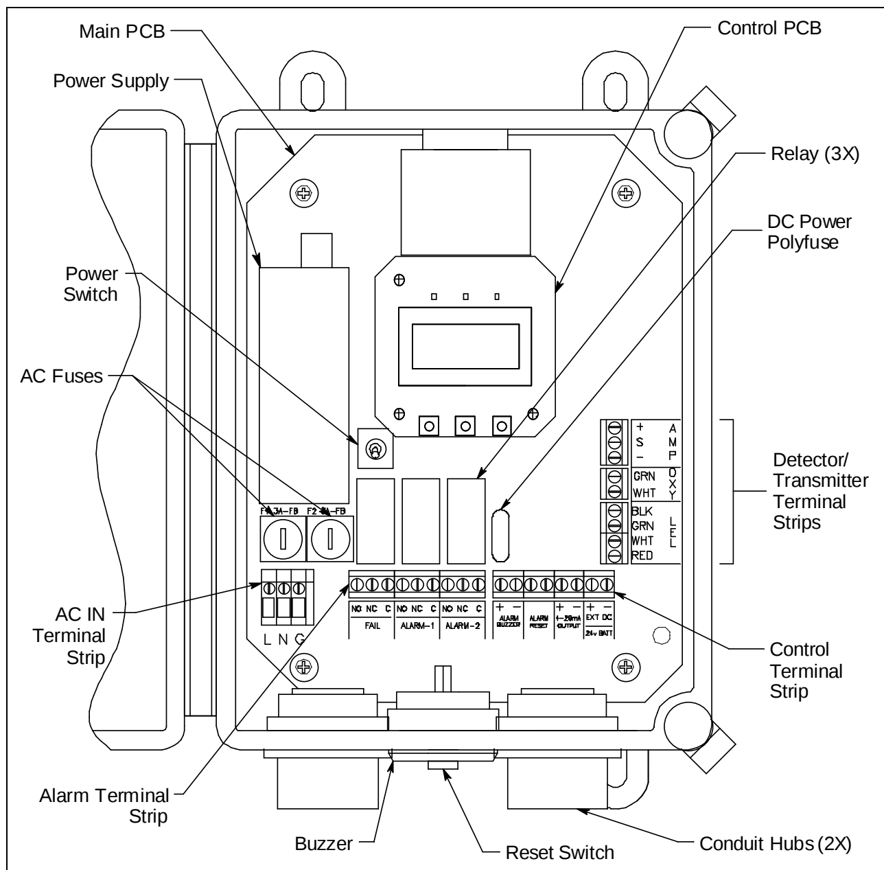
Figure 1: Beacon 110 Component Location
