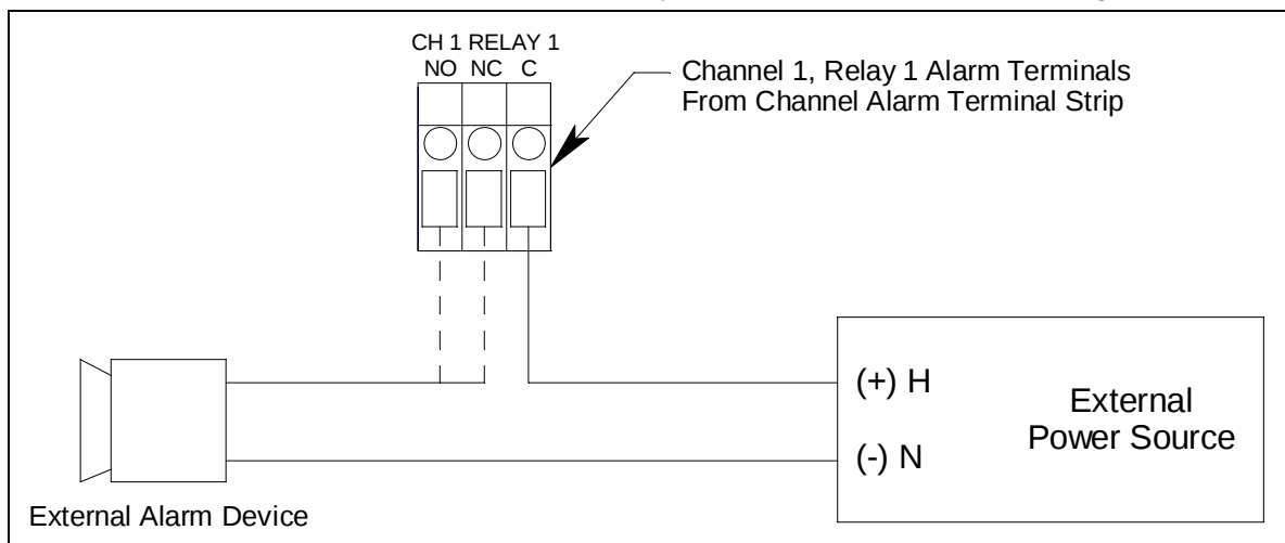
Figure 13: External Alarm Wiring
