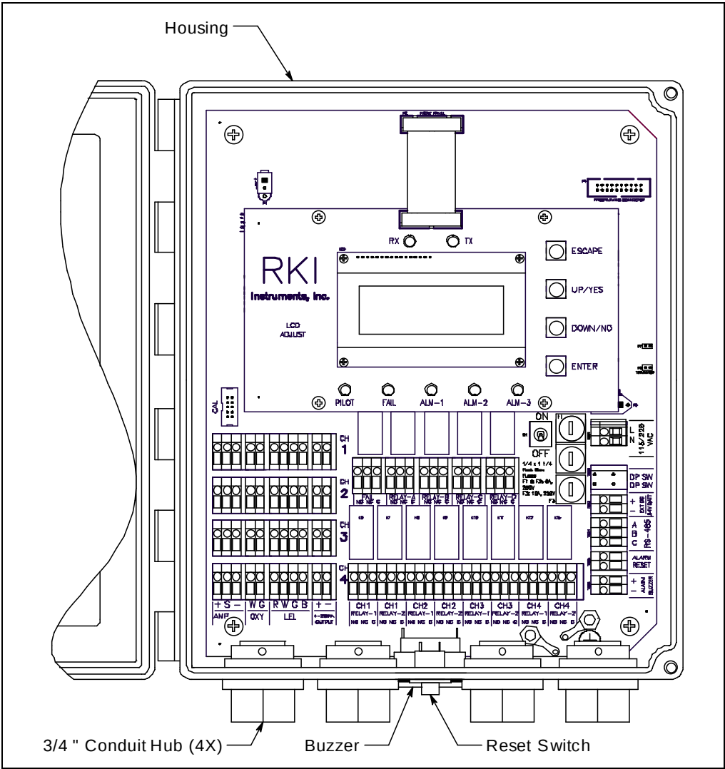
Figure 1: External Component Location
