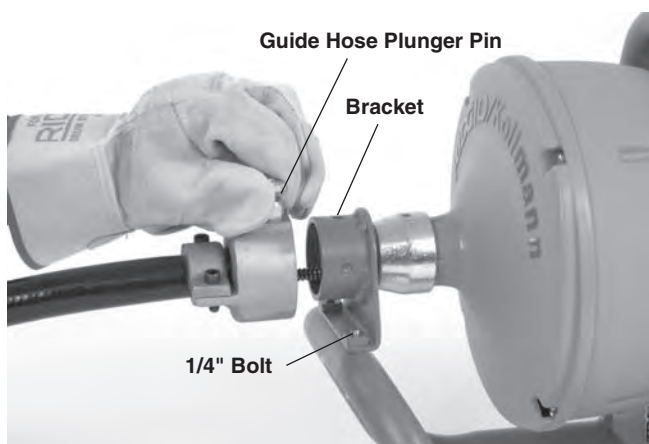
Figure 4 – Mounting Guide Hose to K-40
