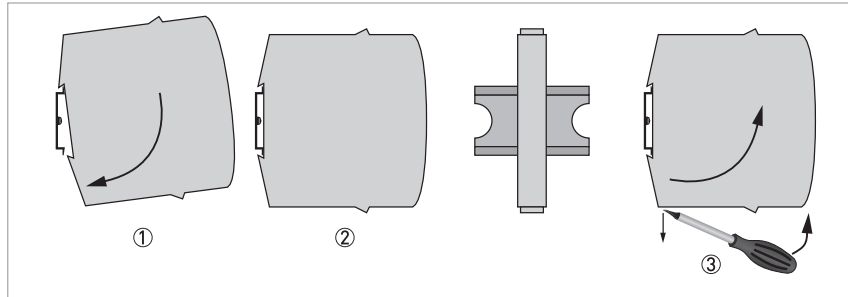
Figure 3-2: Rail installation
