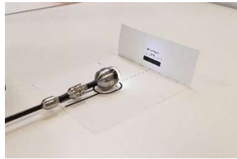
Fig. 49: Calibration with calibration template
