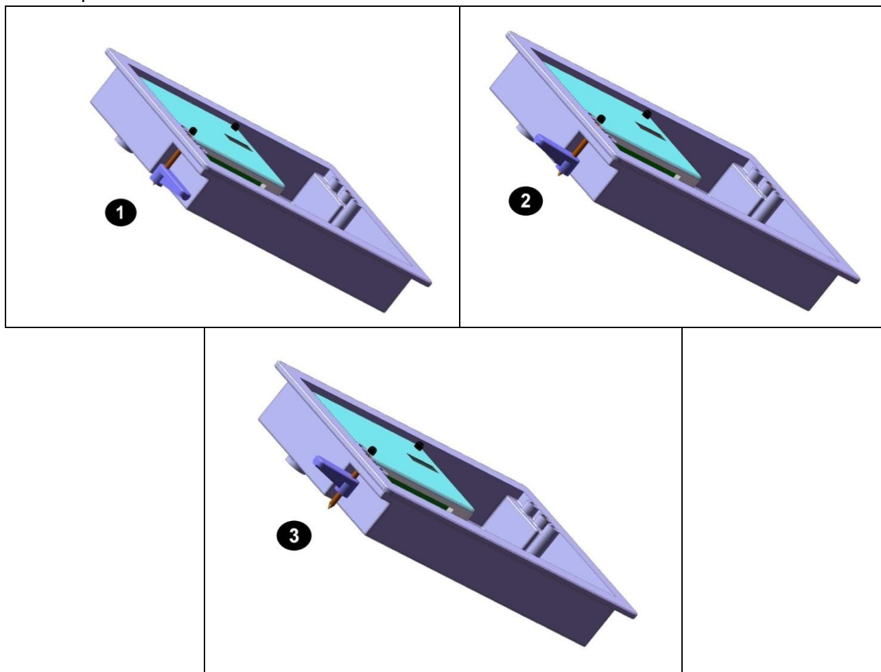
Figure 4: Enclosure installation
