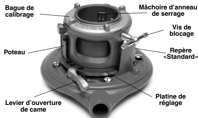
Figure 1 – Fileteuse 65R-C
