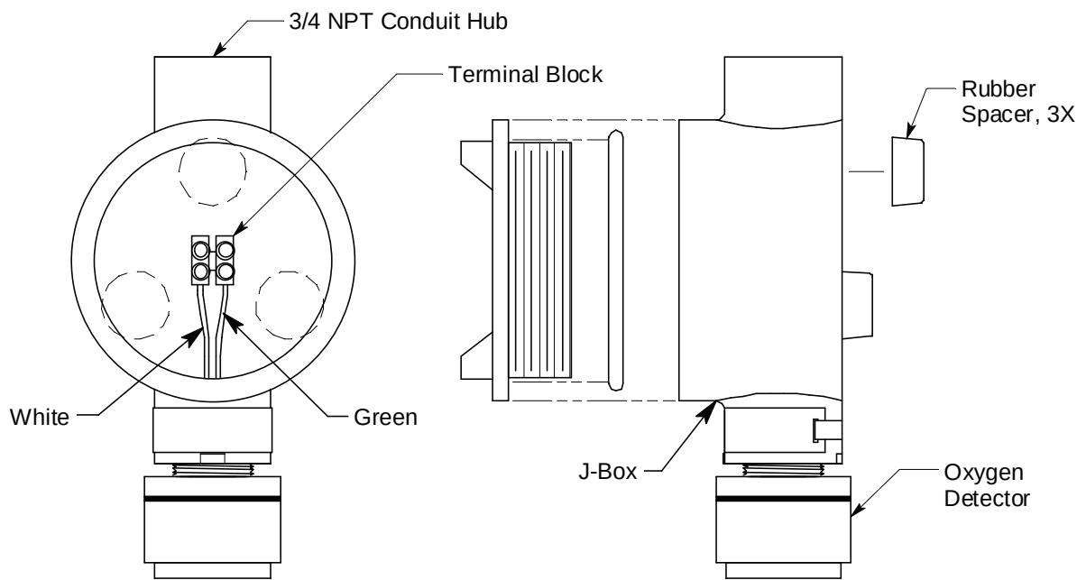
Figure 1: 65-2497RK Component Location
