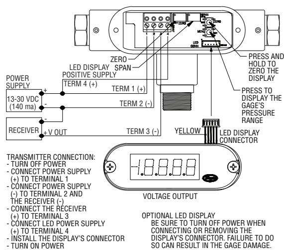
Fig. G: Voltage output with optional LED display
