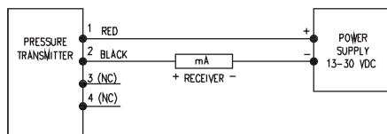
Fig. C: Current output connection
