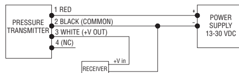
Fig. F: Voltage output connection
