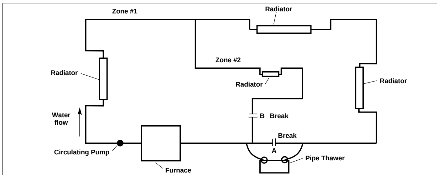
Figure 7 – Multi Zoned System
