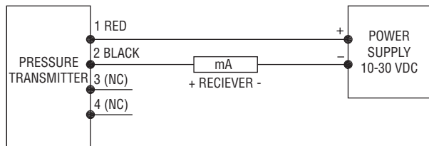
Fig. A: Current output connection
