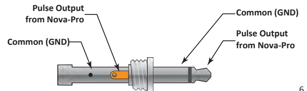
Figure 4 Output Connector Detail (Mono plug)
