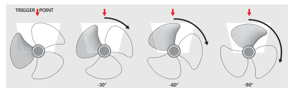
Figure 9 Triggered Phase
