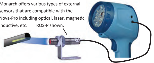
Figure 6 Strobe with External Sensor
